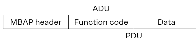
Structure of a Modbus message for Modbus TCP
