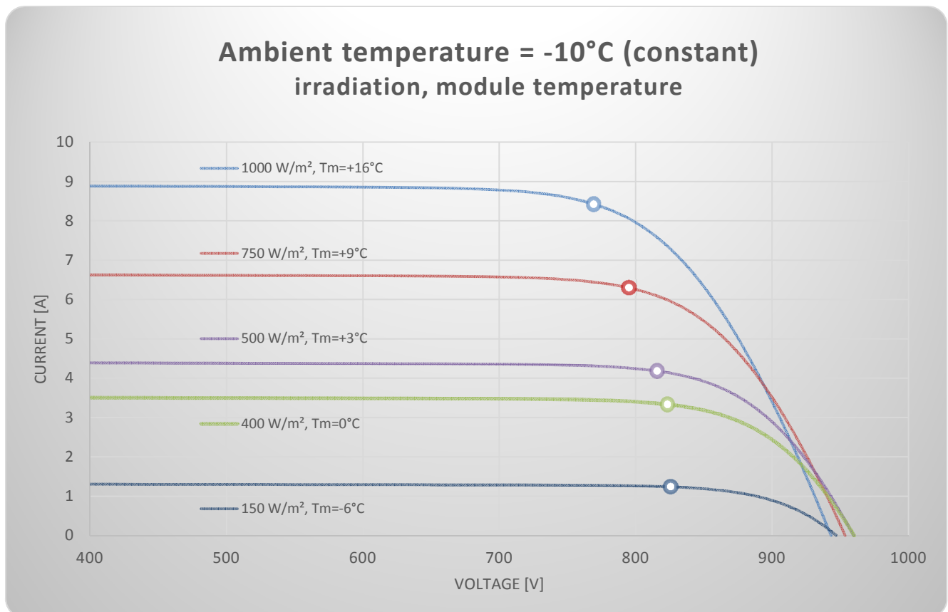
Figure 1: Characteristics T_a=-10\text{ °C} (source: internal analysis - Fronius International GmbH)
